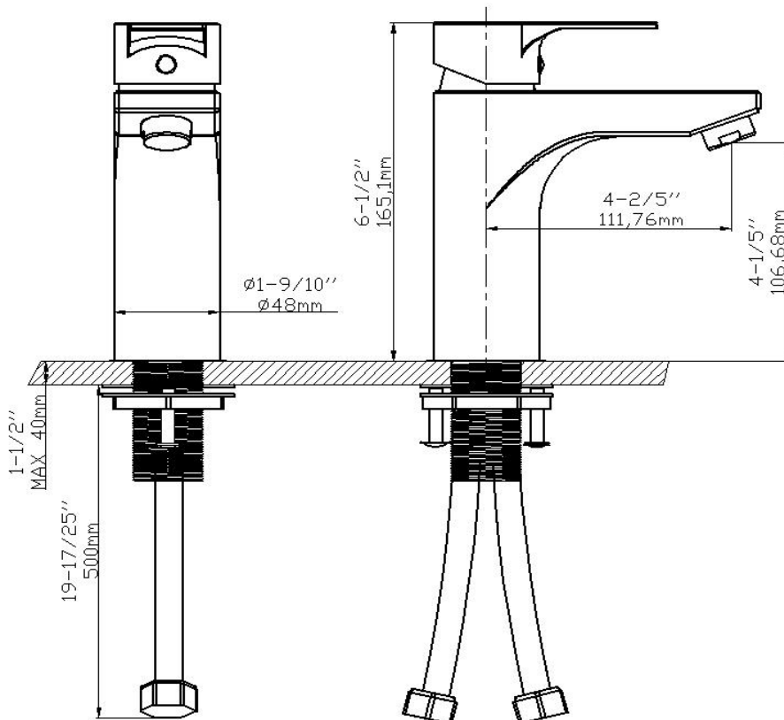
CRITICAL DIMENSIONS
